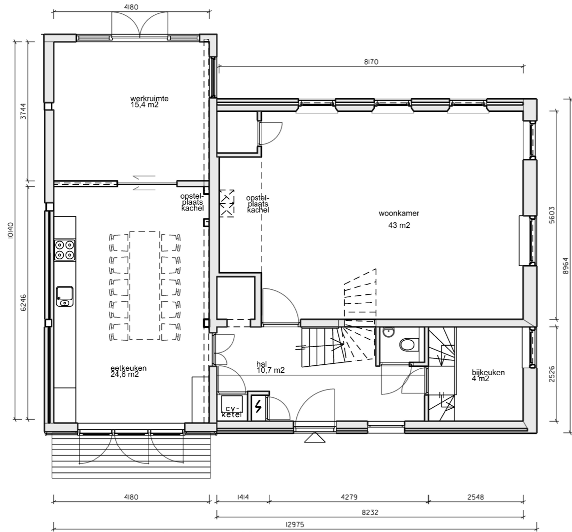
Begane grond (108 m 2 GO)
